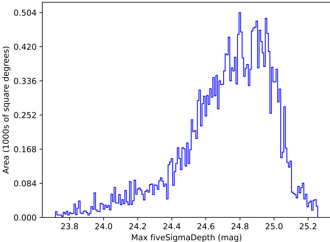
baseline_v3.0_10yrs Yr 1 all bands: Max fiveSigmaDepth
