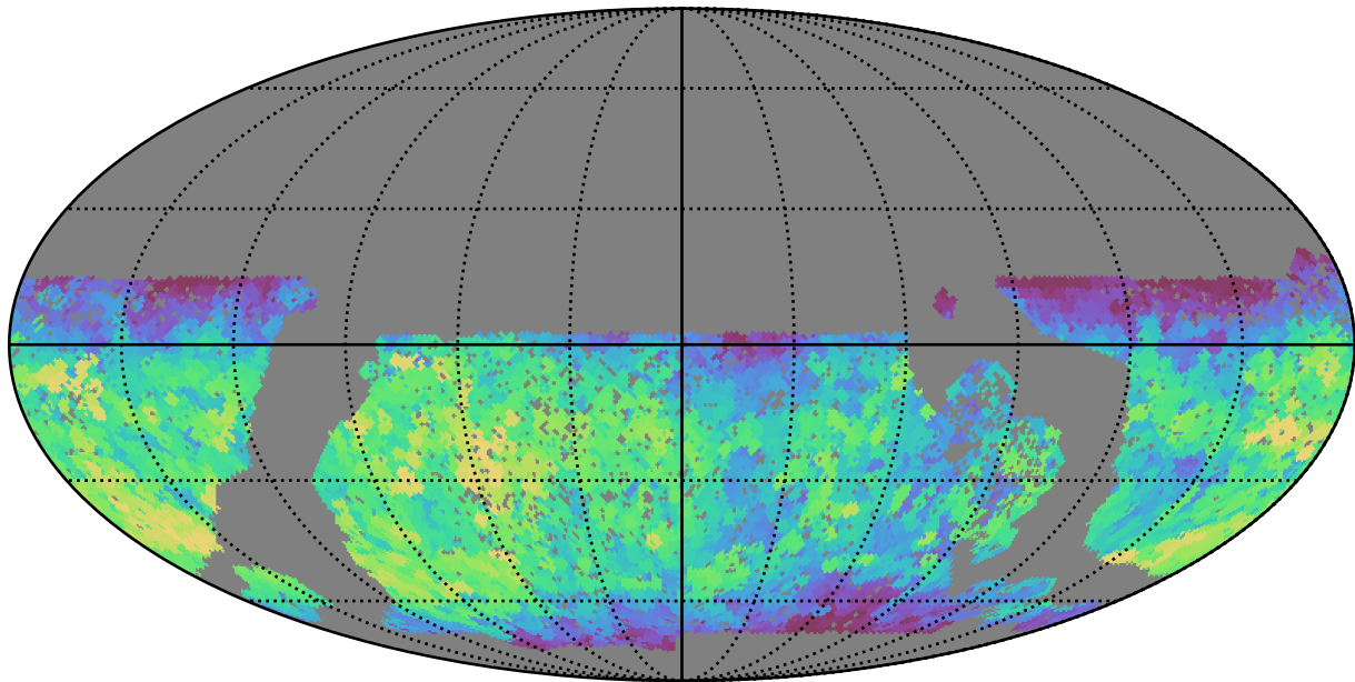
baseline_v3.0_10yrs WFD z band: Max fiveSigmaDepth
