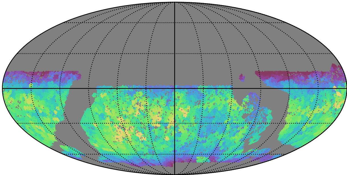
baseline_v3.0_10yrs WFD y band: Max fiveSigmaDepth
