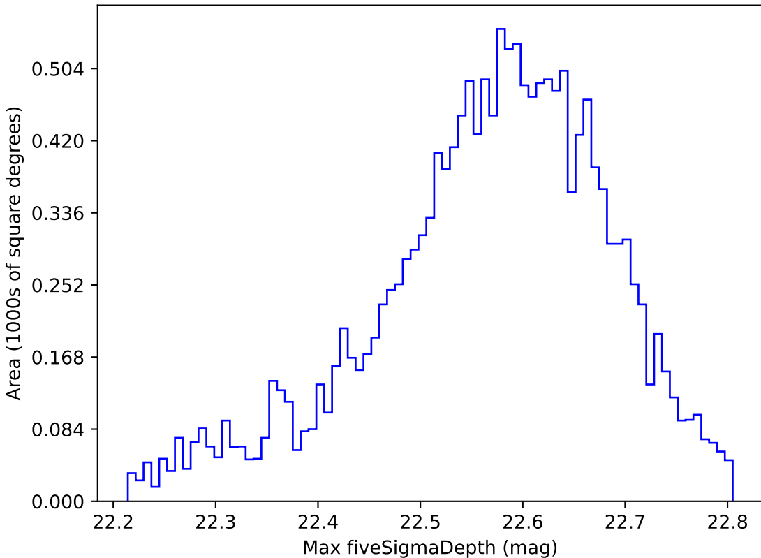
baseline_v3.0_10yrs WFD y band: Max fiveSigmaDepth
