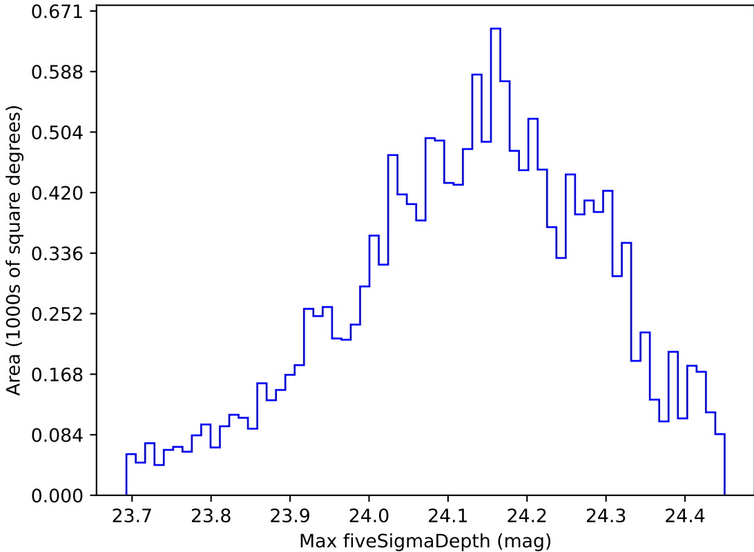
baseline_v3.0_10yrs WFD u band: Max fiveSigmaDepth
