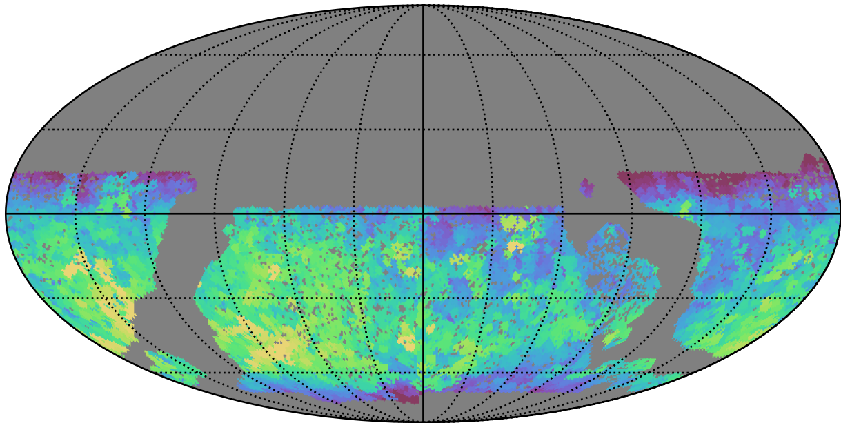
baseline_v3.0_10yrs WFD r band: Max fiveSigmaDepth
