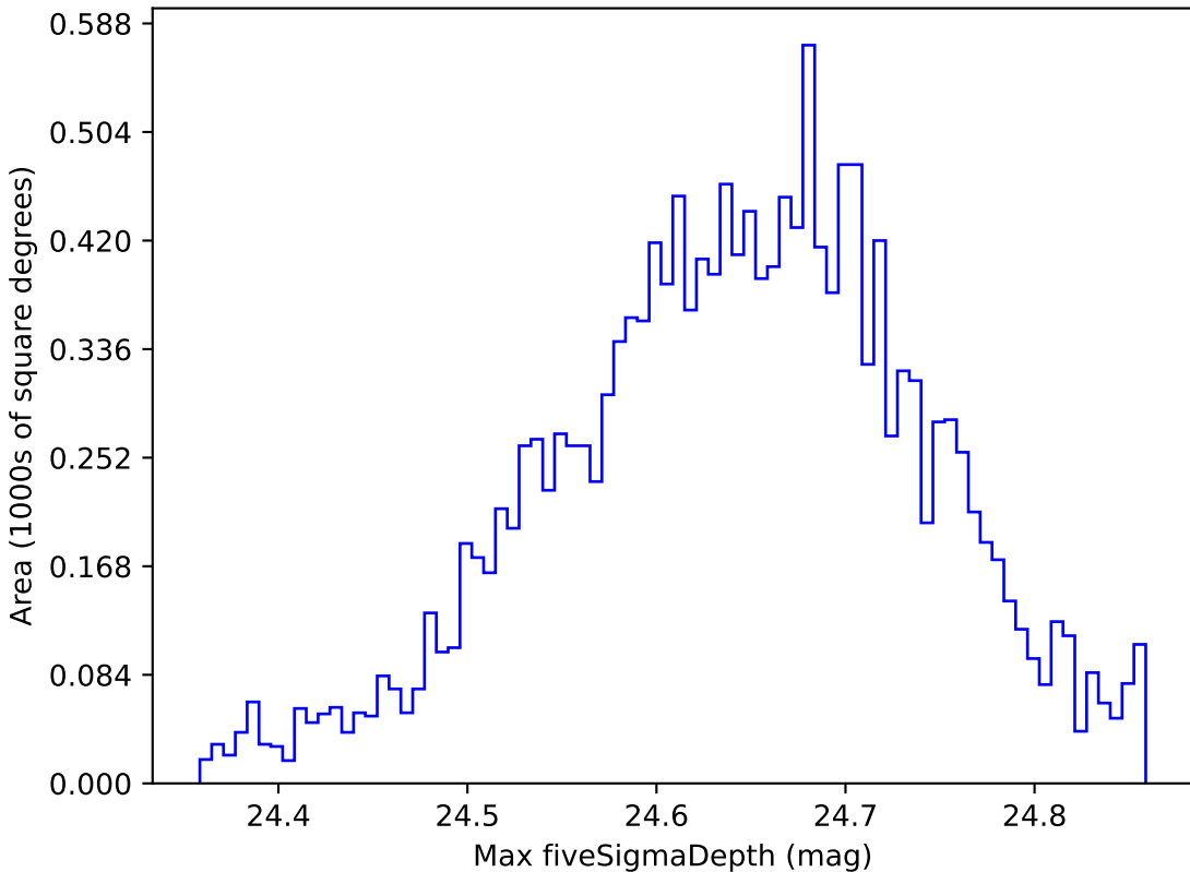
baseline_v3.0_10yrs WFD r band: Max fiveSigmaDepth
