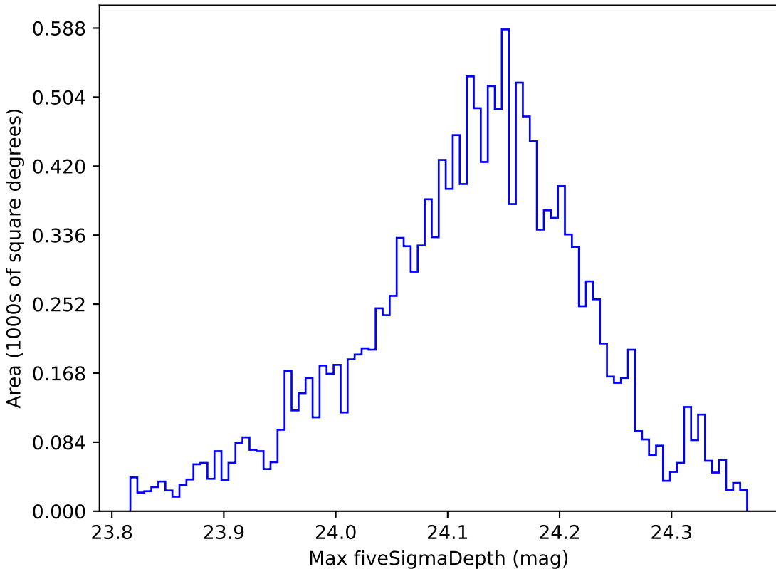
baseline_v3.0_10yrs WFD i band: Max fiveSigmaDepth
