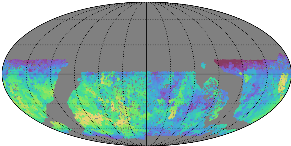
baseline_v3.0_10yrs WFD g band: Max fiveSigmaDepth
