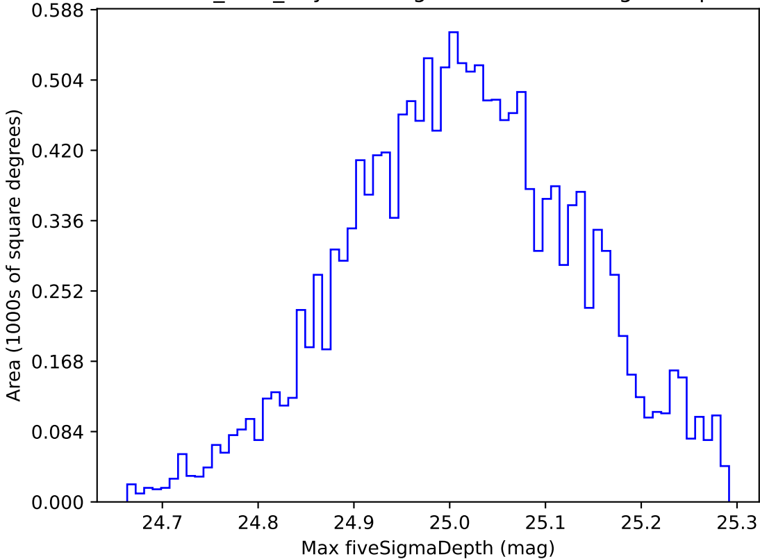
baseline_v3.0_10yrs WFD g band: Max fiveSigmaDepth
