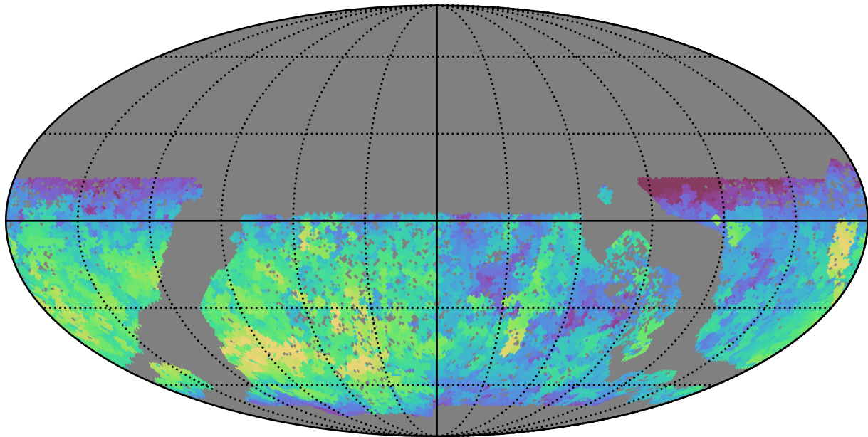
baseline_v3.0_10yrs WFD all bands: Max fiveSigmaDepth
