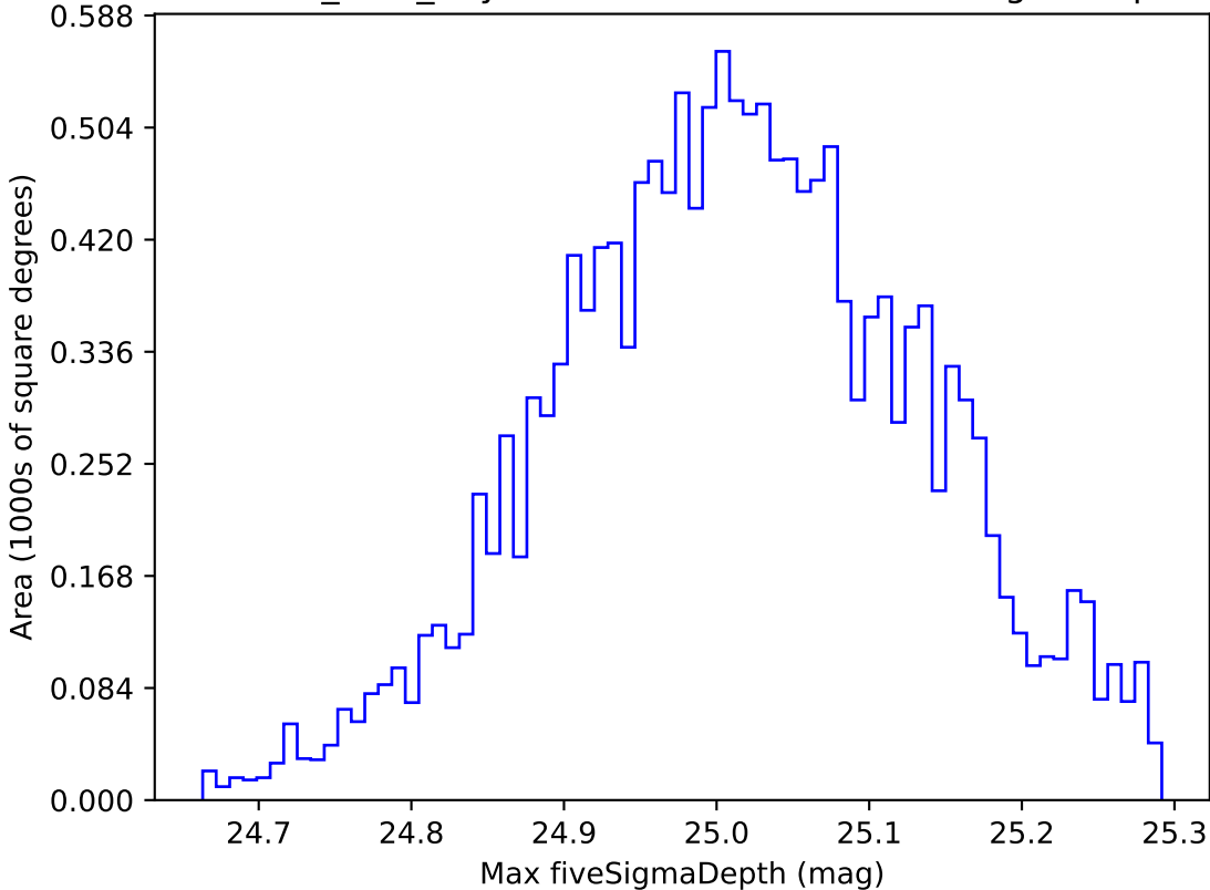
baseline_v3.0_10yrs WFD all bands: Max fiveSigmaDepth
