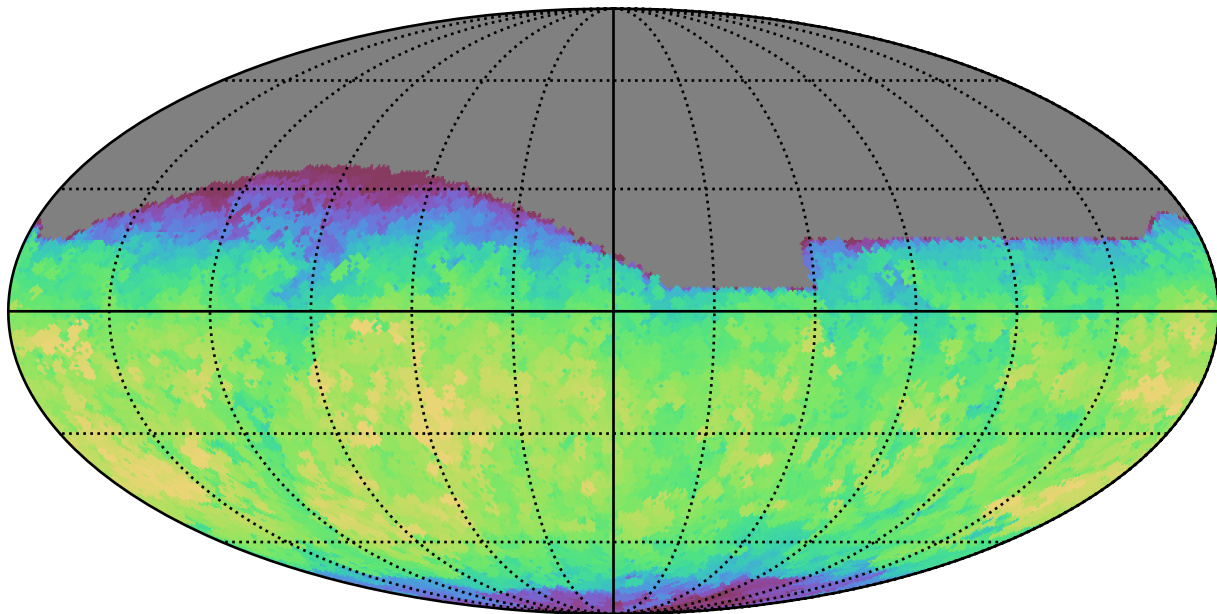
baseline_v3.0_10yrs All sky z band: Max fiveSigmaDepth
