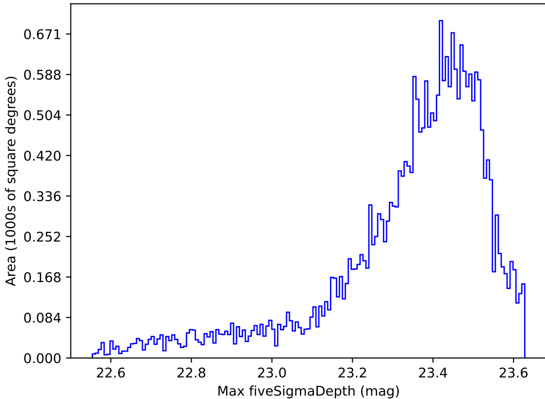
baseline_v3.0_10yrs All sky z band: Max fiveSigmaDepth
