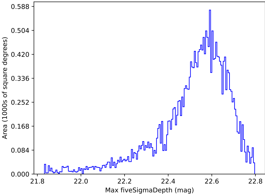
baseline_v3.0_10yrs All sky y band: Max fiveSigmaDepth
