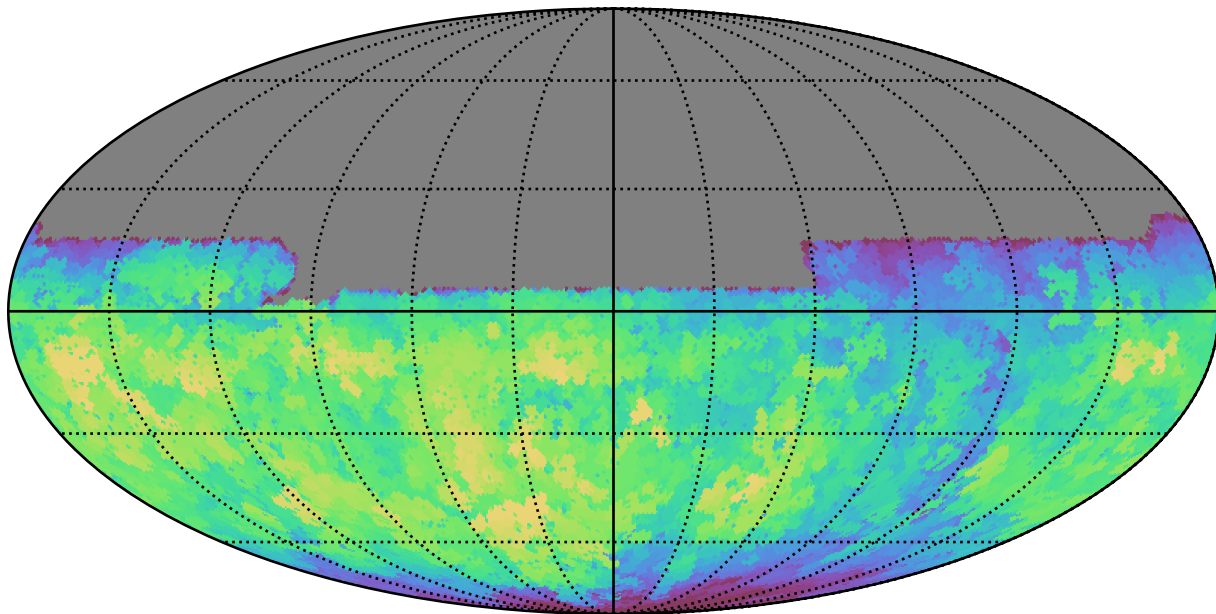
baseline_v3.0_10yrs All sky u band: Max fiveSigmaDepth
