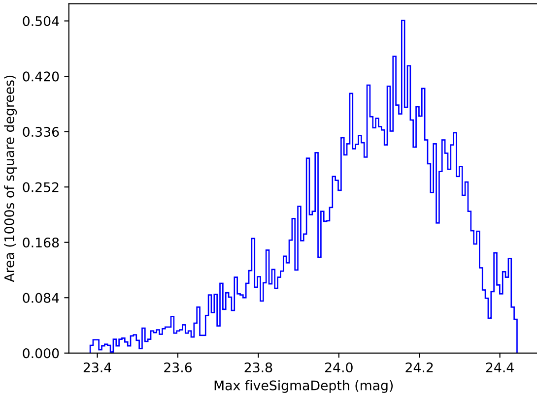
baseline_v3.0_10yrs All sky u band: Max fiveSigmaDepth
