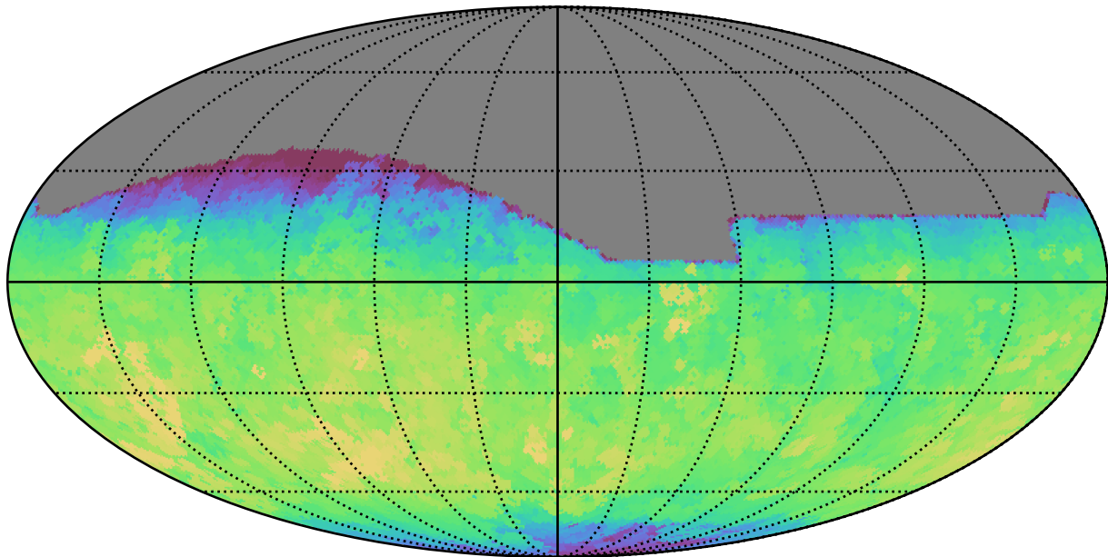
baseline_v3.0_10yrs All sky r band: Max fiveSigmaDepth
