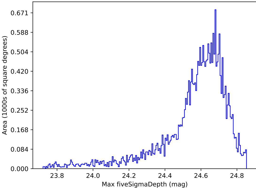
baseline_v3.0_10yrs All sky r band: Max fiveSigmaDepth
