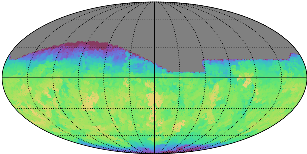
baseline_v3.0_10yrs All sky i band: Max fiveSigmaDepth
