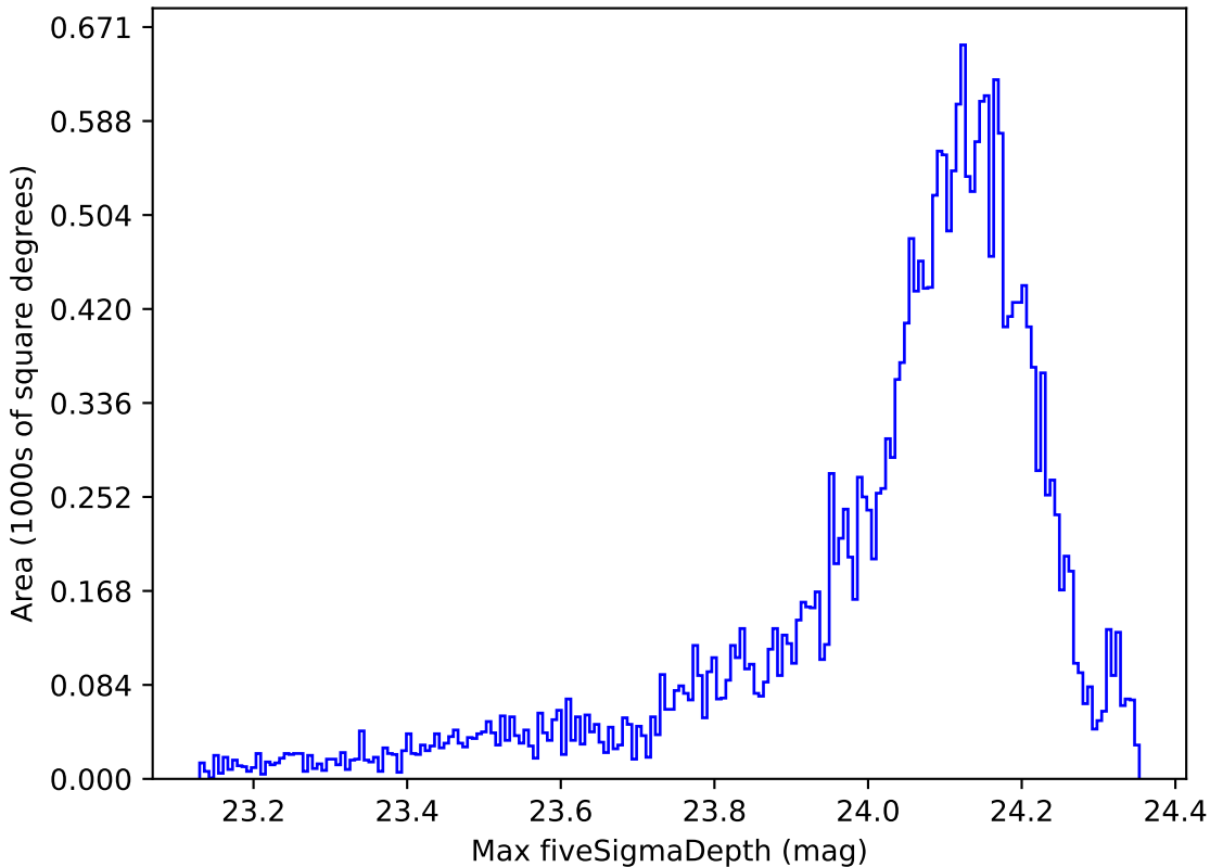
baseline_v3.0_10yrs All sky i band: Max fiveSigmaDepth
