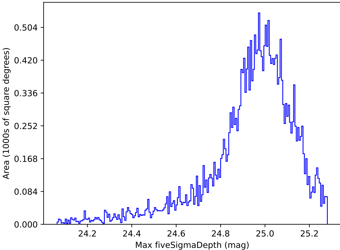
baseline_v3.0_10yrs All sky g band: Max fiveSigmaDepth
