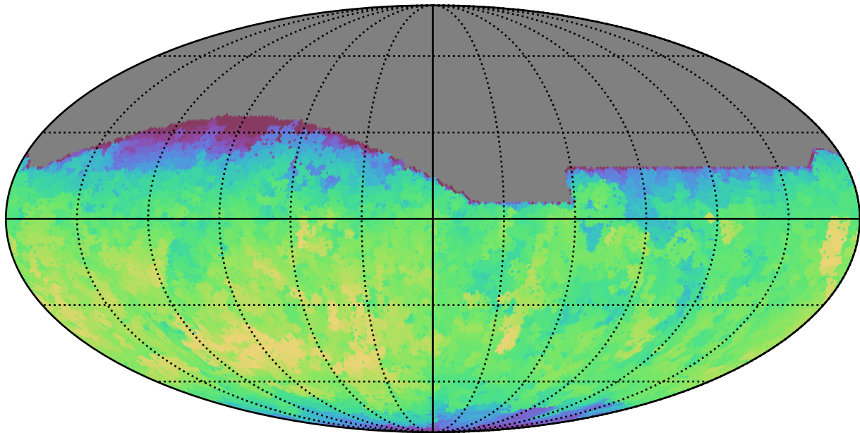
baseline_v3.0_10yrs All sky all bands: Max fiveSigmaDepth
