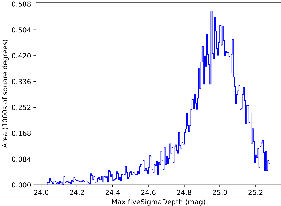
baseline_v3.0_10yrs All sky all bands: Max fiveSigmaDepth
