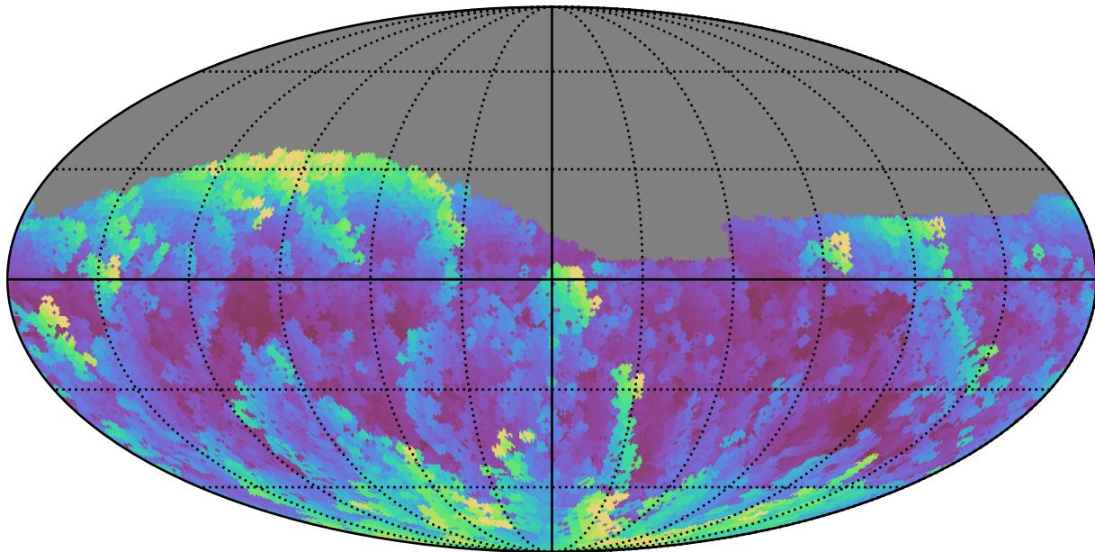
baseline_v3.0_10yrs Yr 1 z band: Max airmass
