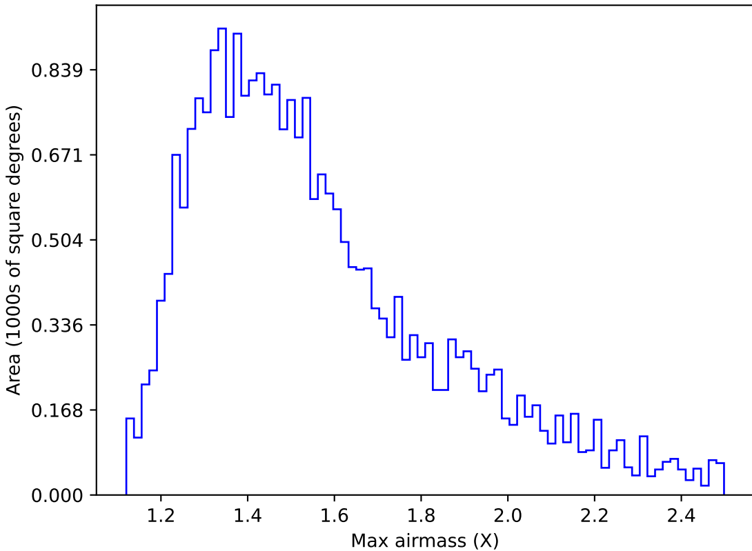
baseline_v3.0_10yrs Yr 1 z band: Max airmass
