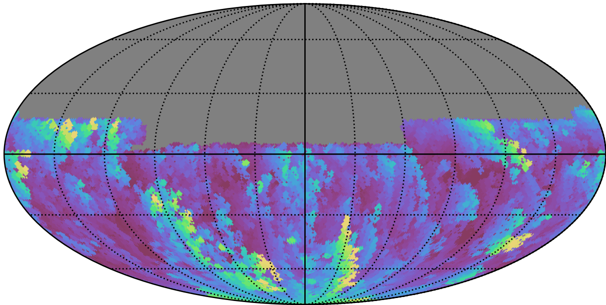
baseline_v3.0_10yrs Yr 1 y band: Max airmass
