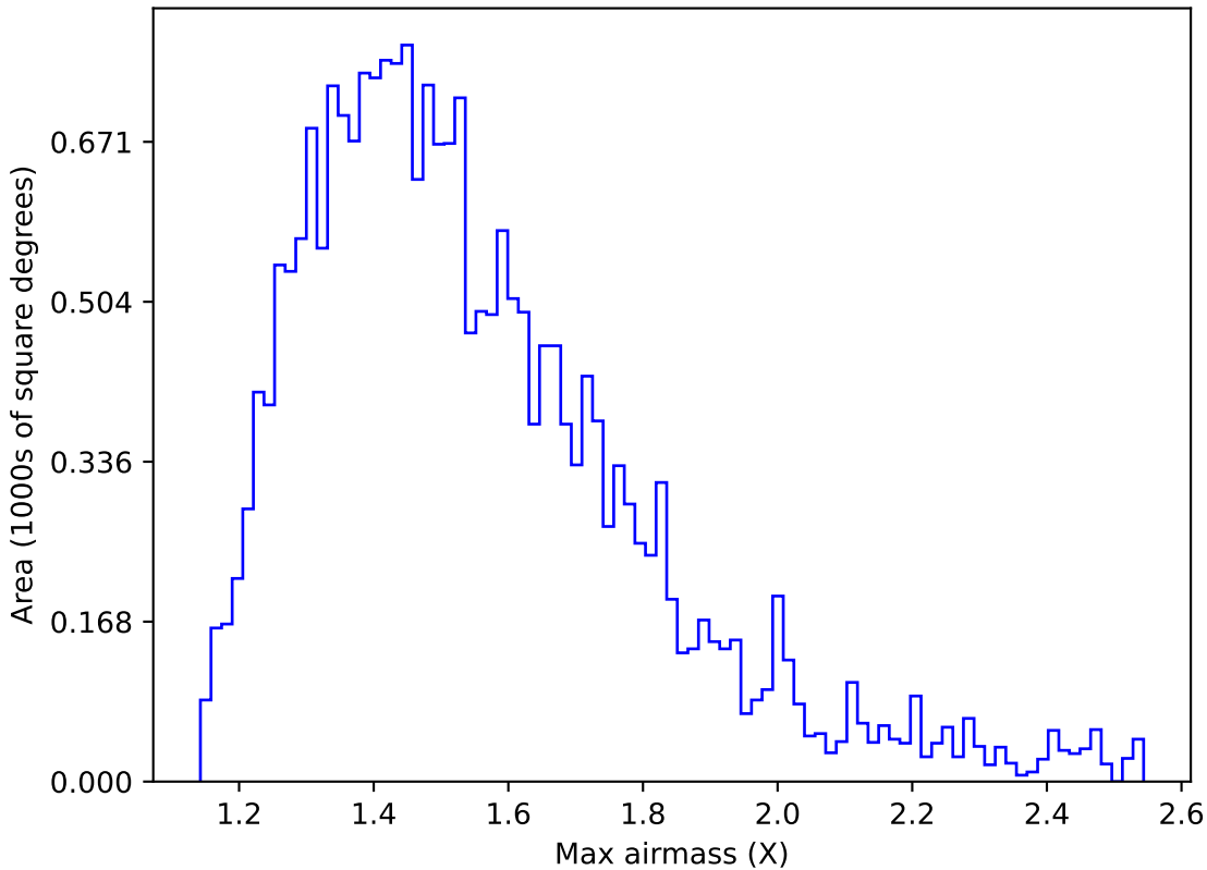
baseline_v3.0_10yrs Yr 1 y band: Max airmass
