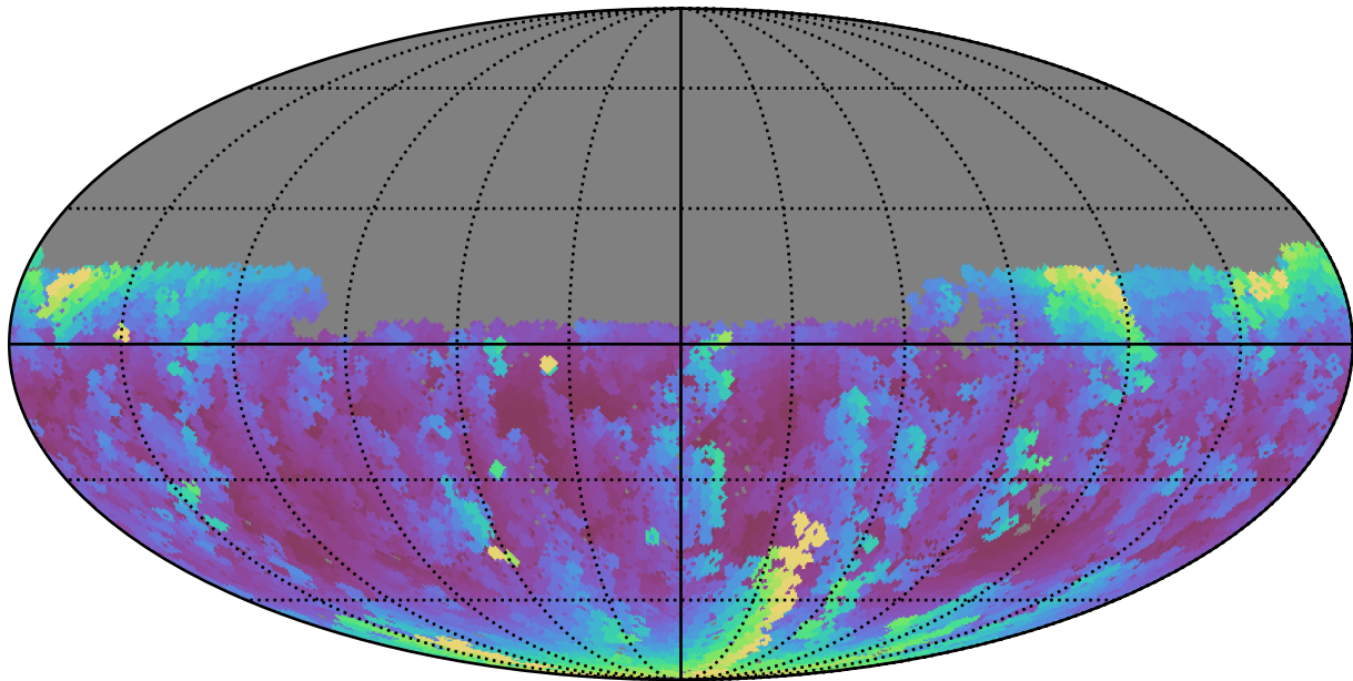
baseline_v3.0_10yrs Yr 1 u band: Max airmass
