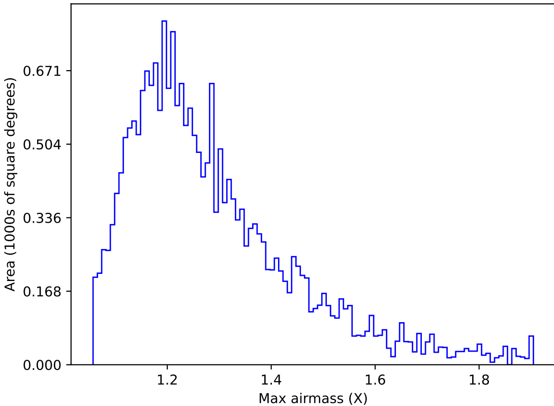
baseline_v3.0_10yrs Yr 1 u band: Max airmass
