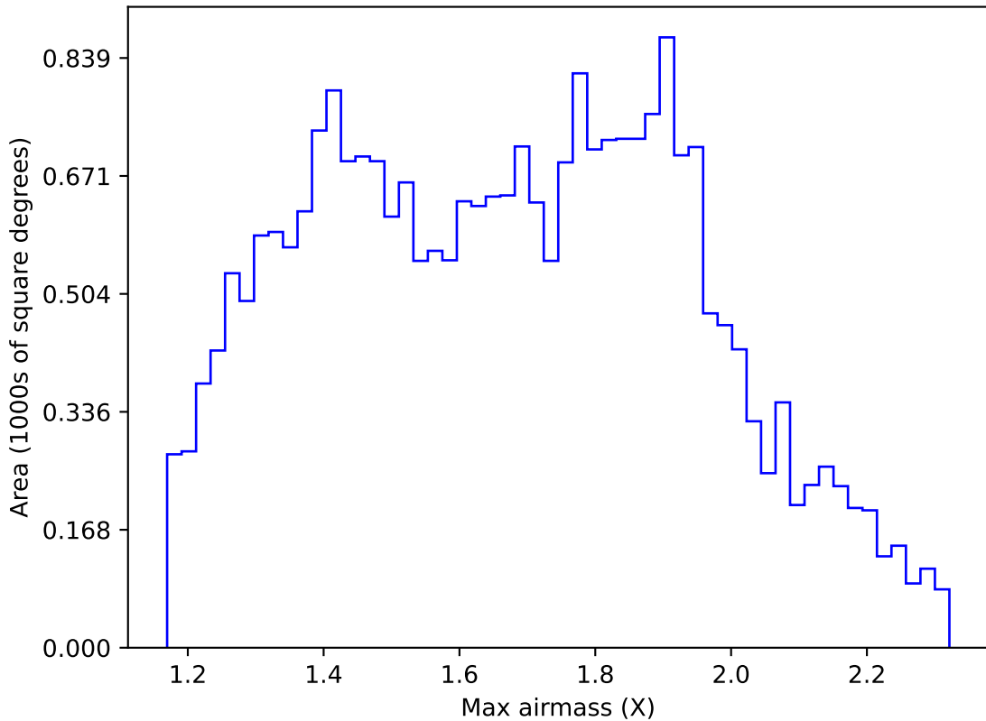
baseline_v3.0_10yrs Yr 1 r band: Max airmass
