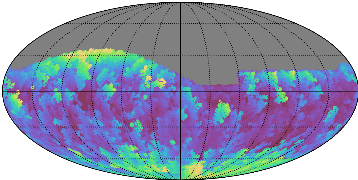
baseline_v3.0_10yrs Yr 1 i band: Max airmass
