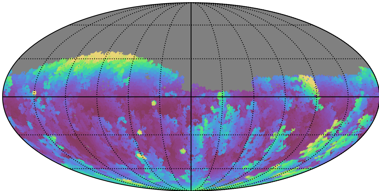
baseline_v3.0_10yrs Yr 1 g band: Max airmass
