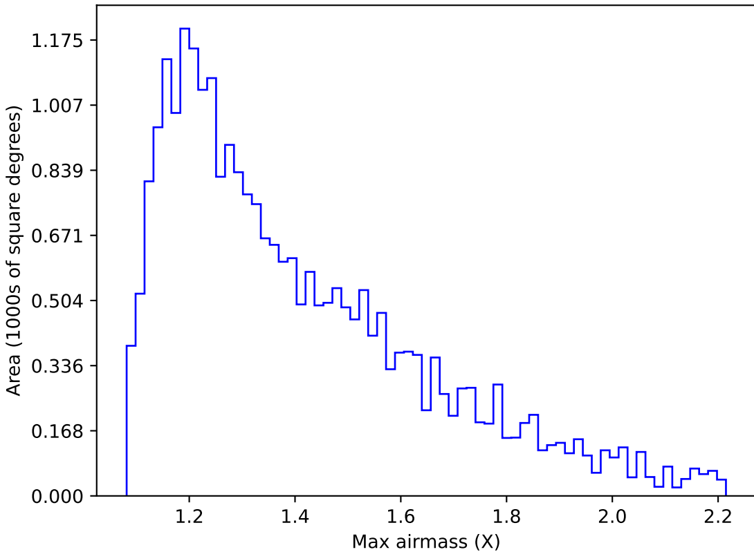
baseline_v3.0_10yrs Yr 1 g band: Max airmass
