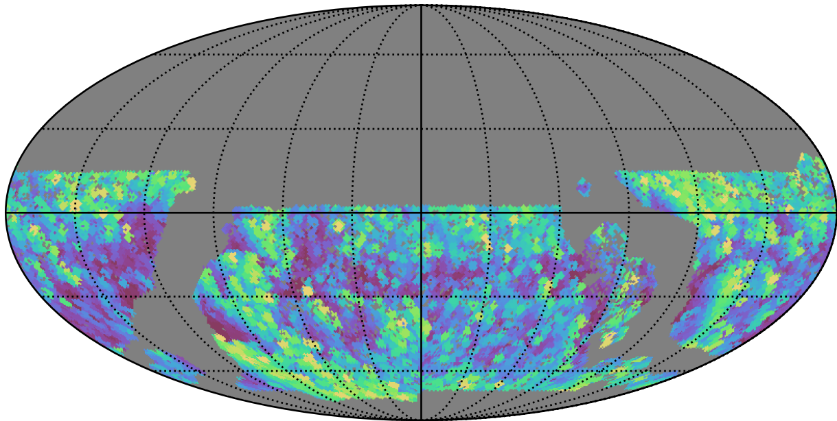
baseline_v3.0_10yrs WFD z band: Max airmass
