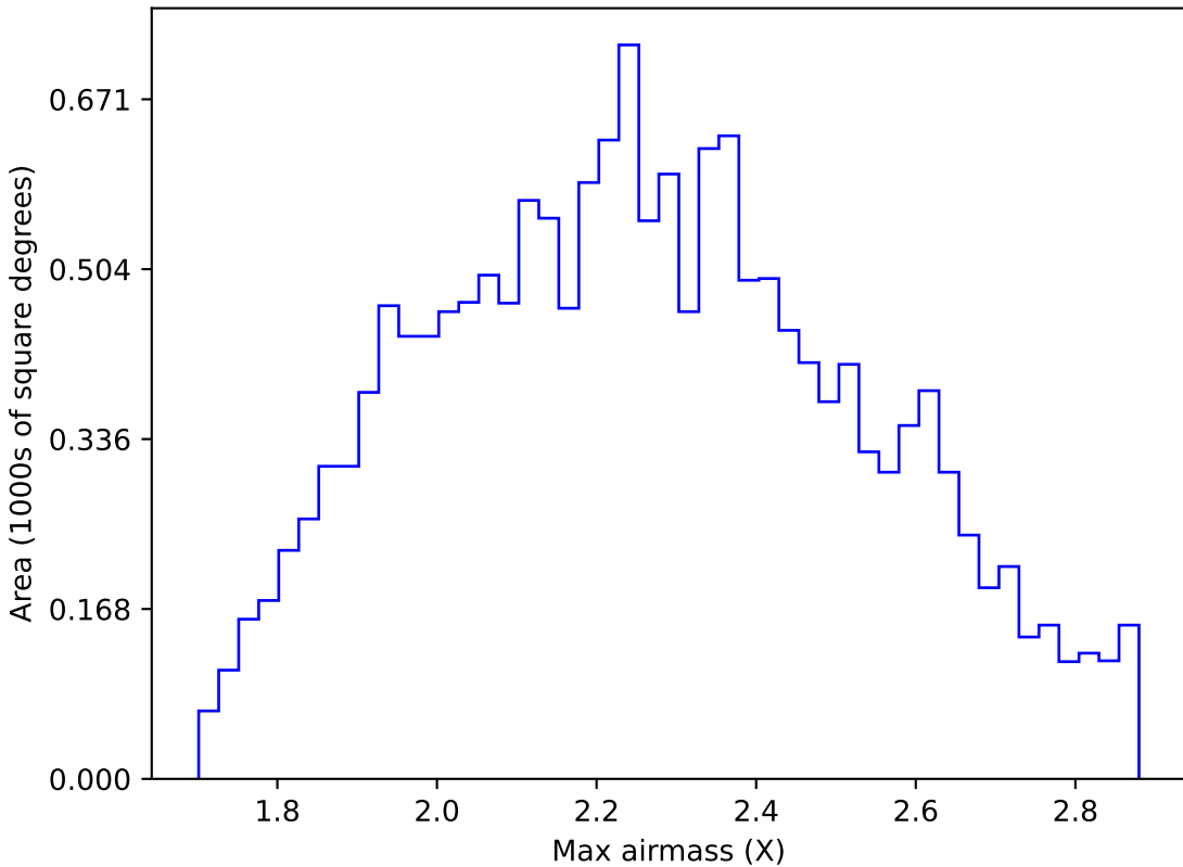
baseline_v3.0_10yrs WFD z band: Max airmass
