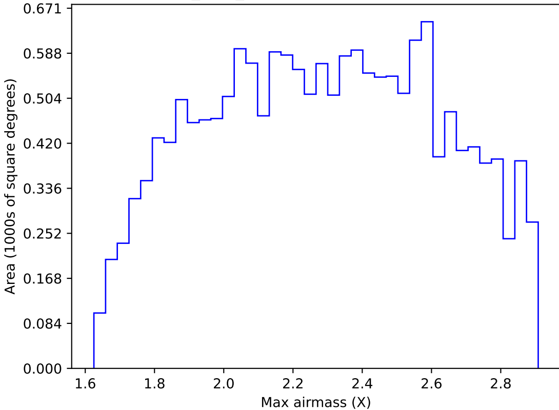
baseline_v3.0_10yrs WFD y band: Max airmass
