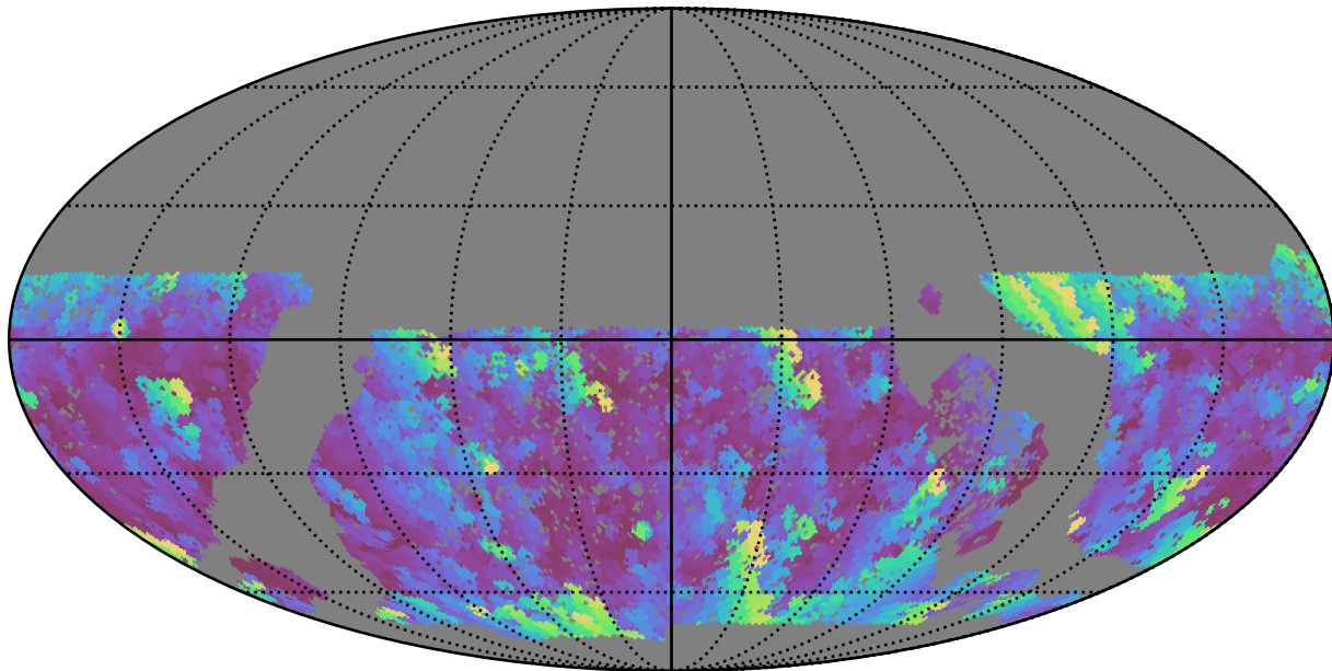
baseline_v3.0_10yrs WFD u band: Max airmass
