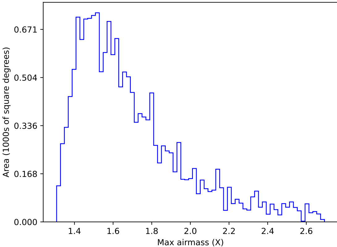
baseline_v3.0_10yrs WFD u band: Max airmass
