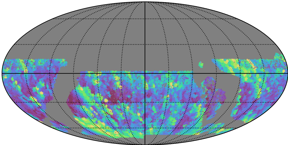
baseline_v3.0_10yrs WFD r band: Max airmass
