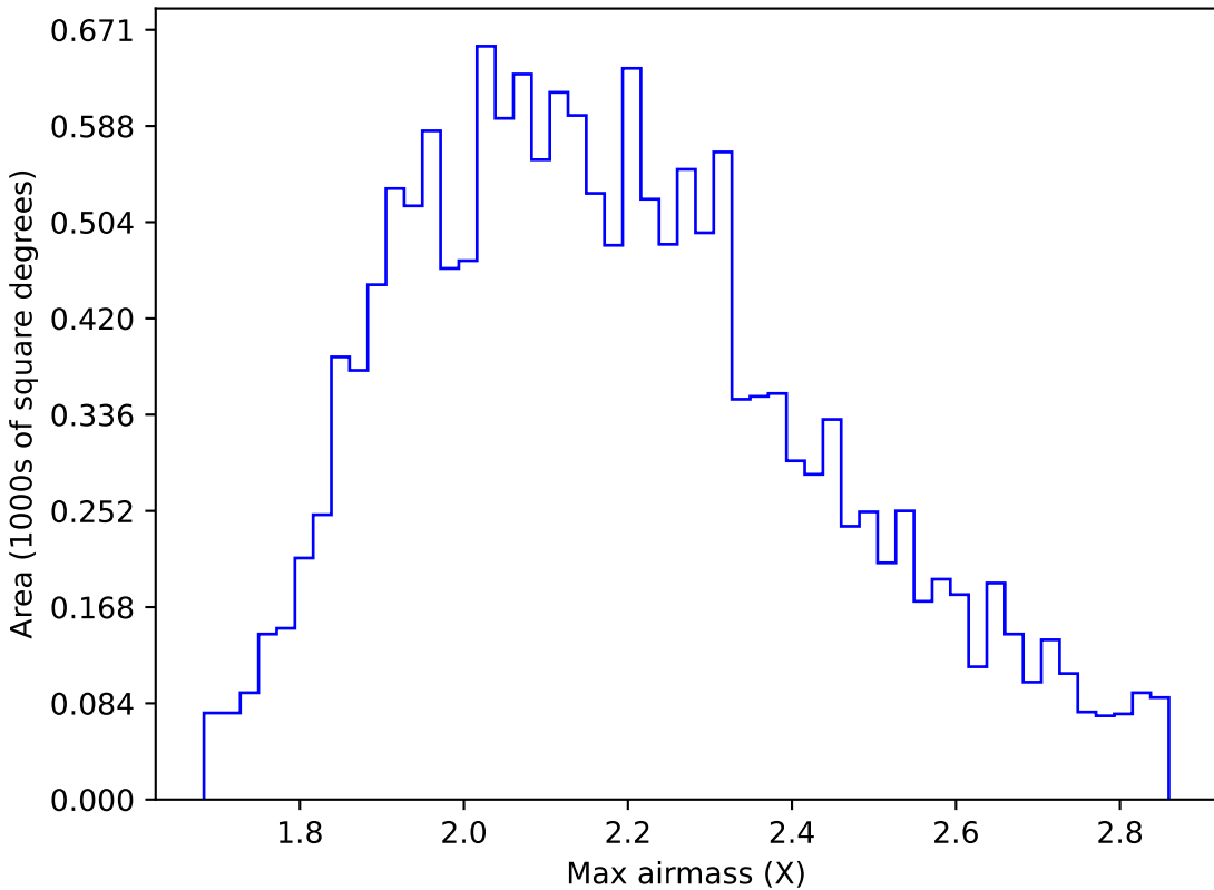
baseline_v3.0_10yrs WFD r band: Max airmass
