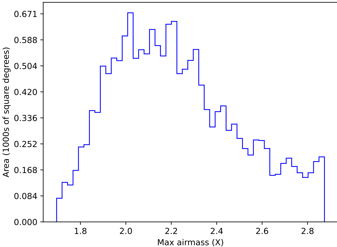
baseline_v3.0_10yrs WFD i band: Max airmass
