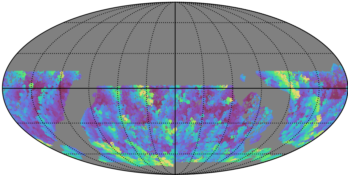
baseline_v3.0_10yrs WFD g band: Max airmass
