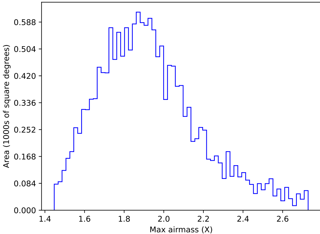
baseline_v3.0_10yrs WFD g band: Max airmass
