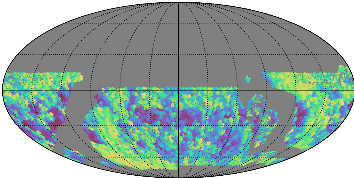
baseline_v3.0_10yrs WFD all bands: Max airmass
