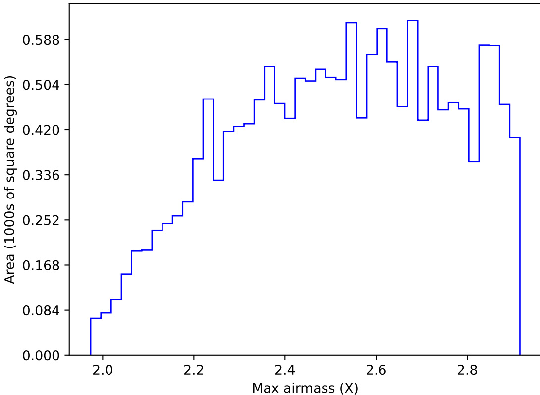
baseline_v3.0_10yrs WFD all bands: Max airmass
