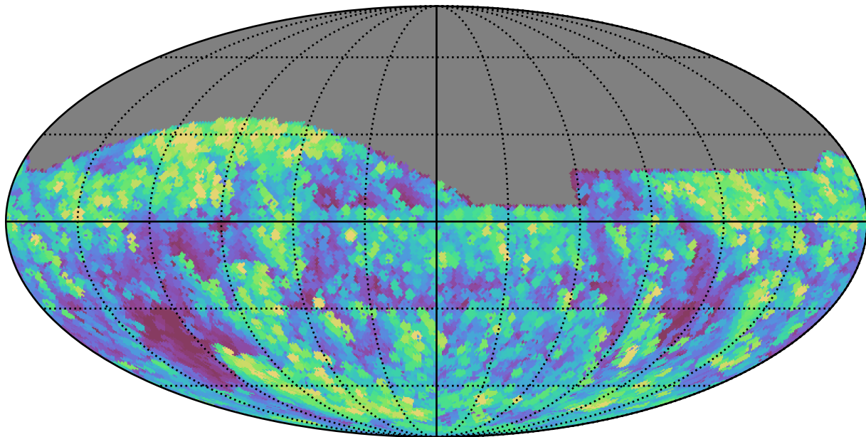
baseline_v3.0_10yrs All sky z band: Max airmass
