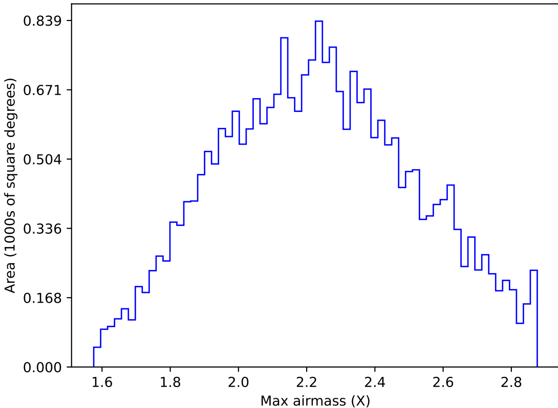
baseline_v3.0_10yrs All sky z band: Max airmass
