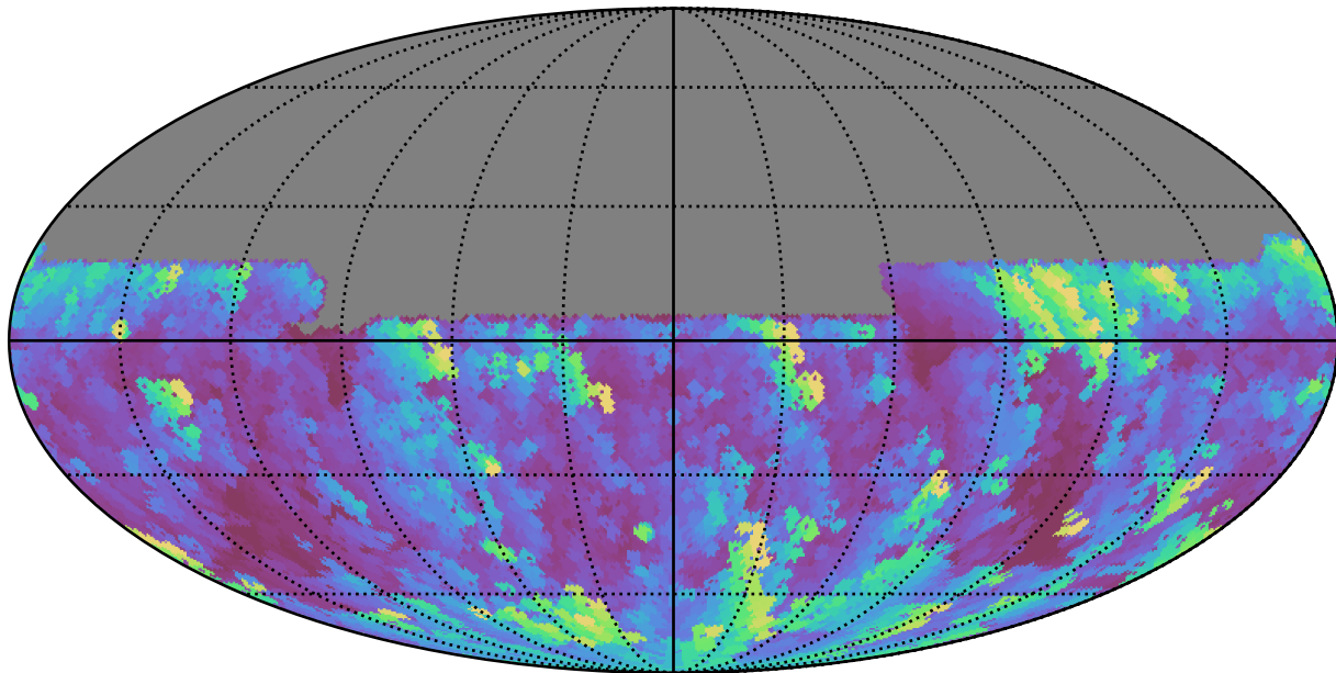
baseline_v3.0_10yrs All sky u band: Max airmass
