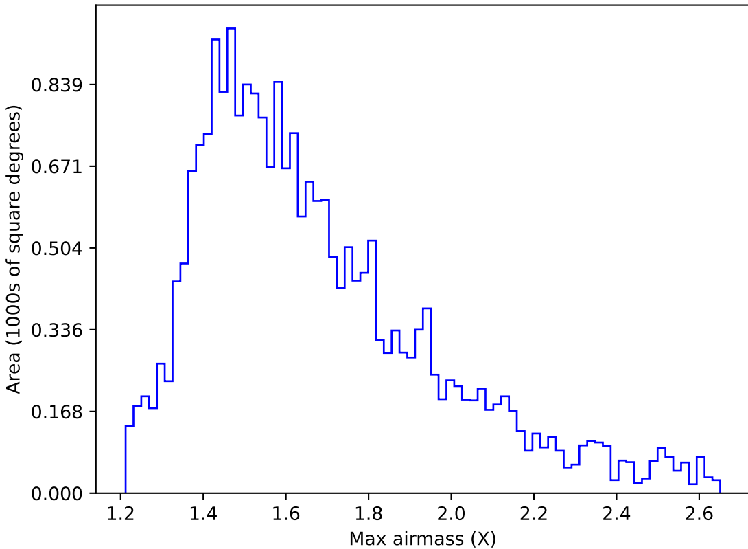
baseline_v3.0_10yrs All sky u band: Max airmass
